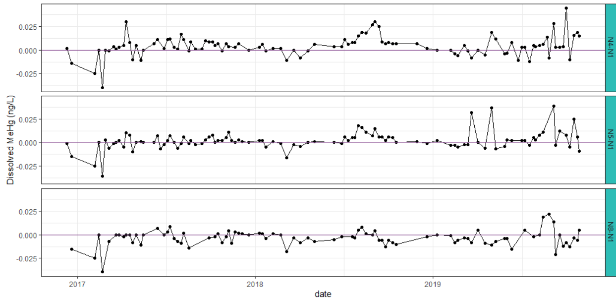
Figure 2: Dissolved methylmercury within (N4), immediately downriver of Muskrat Falls reservoir (N5), and Goose Bay (N8) relative to upriver control (N1 - Grizzle Rapids)
